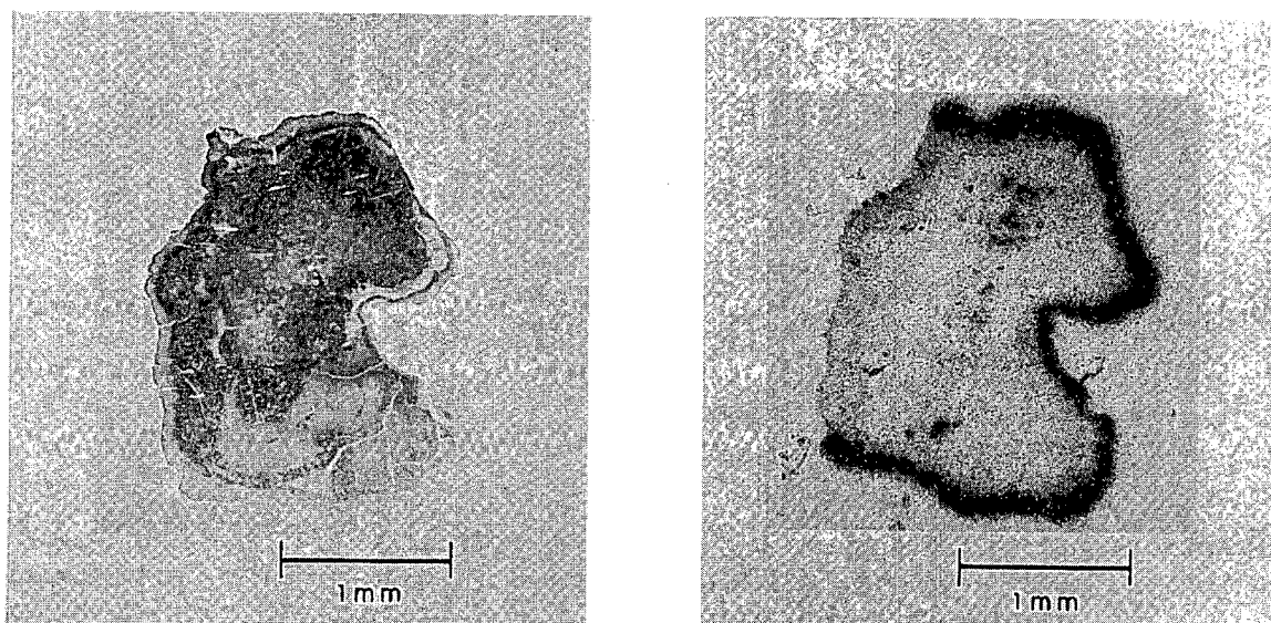
Fig. 4. Photograph (left) and autoradiograph (right) of a thin section of an irregular particle from a ground-surface shot at Bikini. The radioactivity is concentrated on the surface of the particle.
